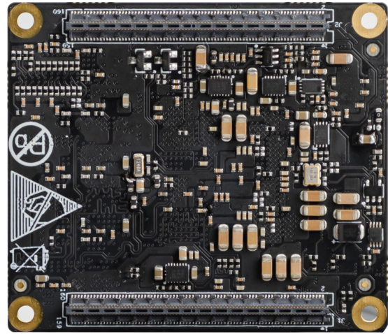
Figure 1-7 MYC-CZU3EG/4EV/5EV-V2 Bottom-view
