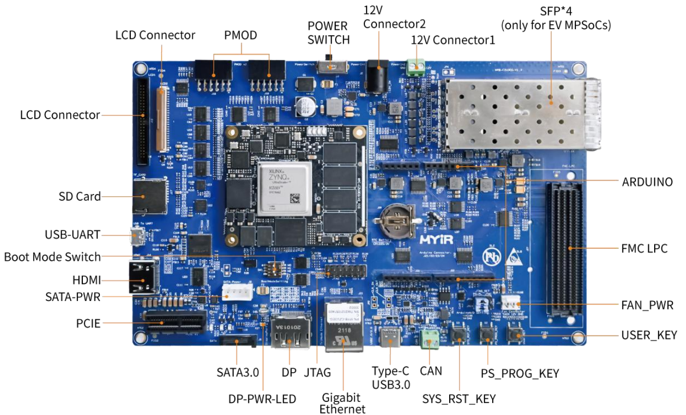
Figure 1-3 MYD-CZU3EG/4EV/5EV-V2 Development Board
