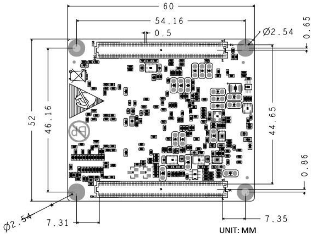
Figure 1-9 Dimension Chart of MYC-CZU3EG/4EV/5EV-V2 (Top-view)
