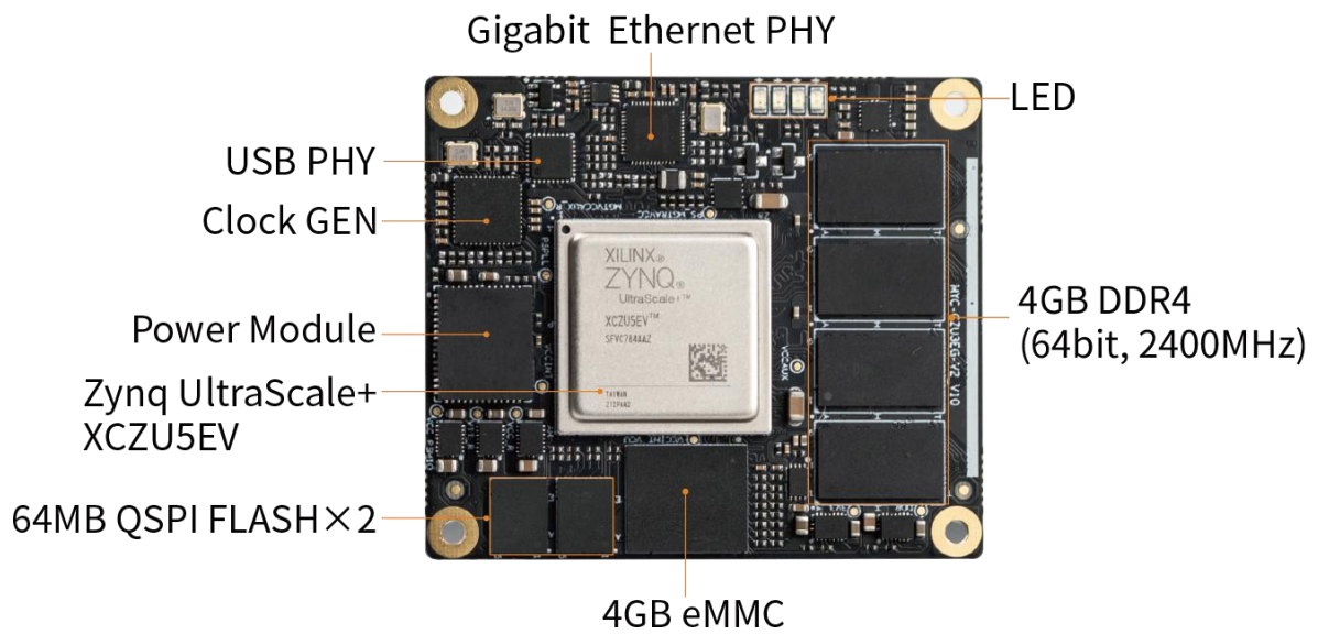
Figure 1-2 MYC-CZU3EG/4EV/5EV-V2 CPU Module
