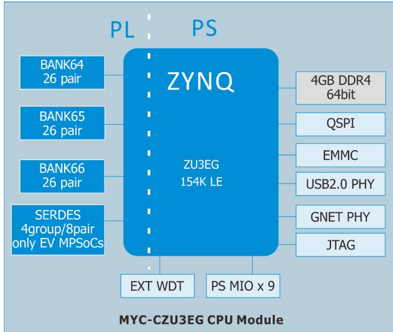
Figure 1-8 Function Block Diagram of MYC-CZU3EG/4EV/5EV-V2
