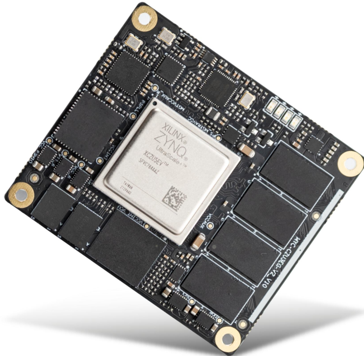
Figure 1-1 MYC-CZU3EG/4EV/5EV-V2 CPU Module
